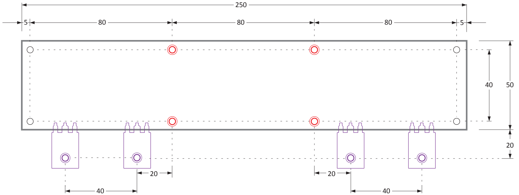
FRONT VIEW Circuit Board Dimensions
