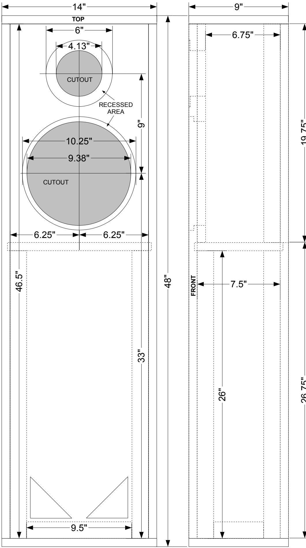
FRONT VIEW
