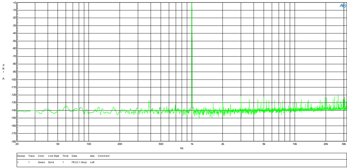
Buffalo 32S Differential output FFT @ 1k. (-117dB THD+N)
