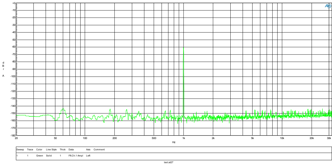
Buffalo 32S Differential Output DNR
