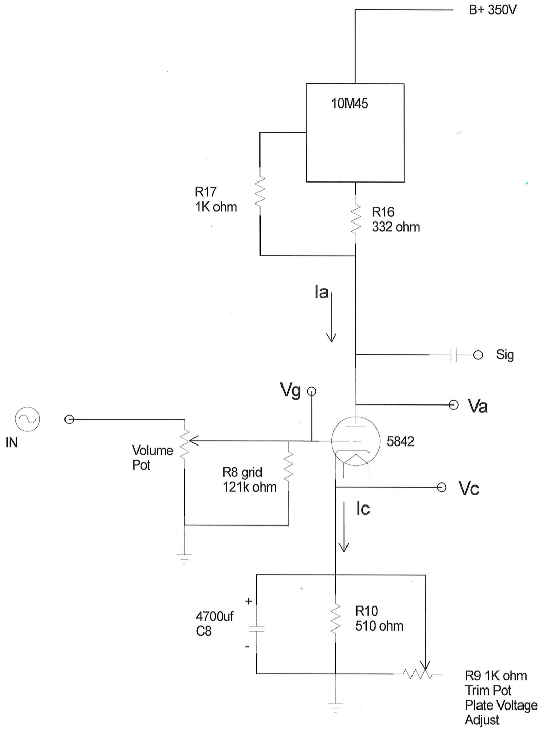
Tube Lab SE Input Stage
