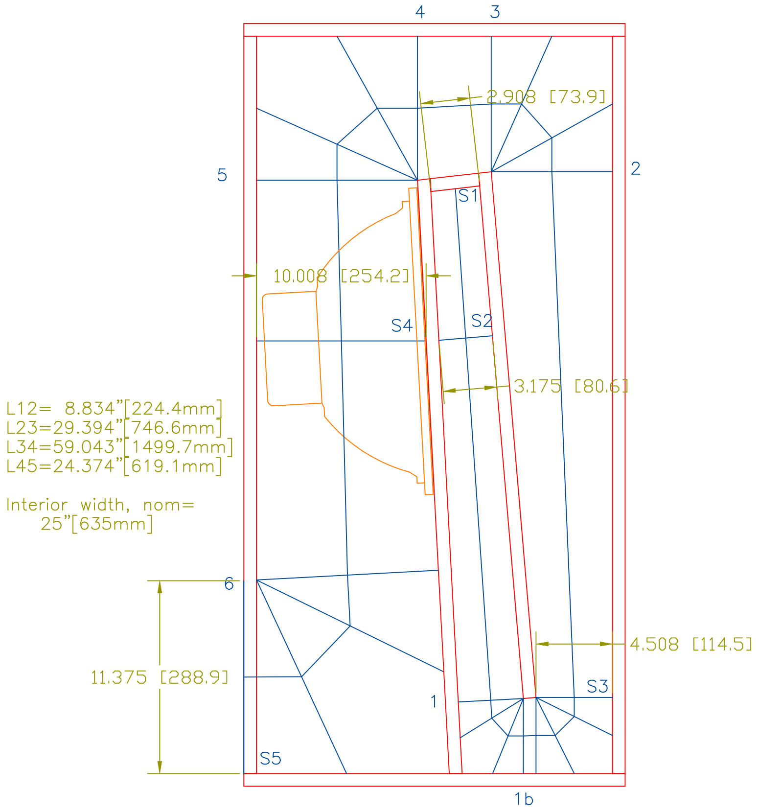
Side view
