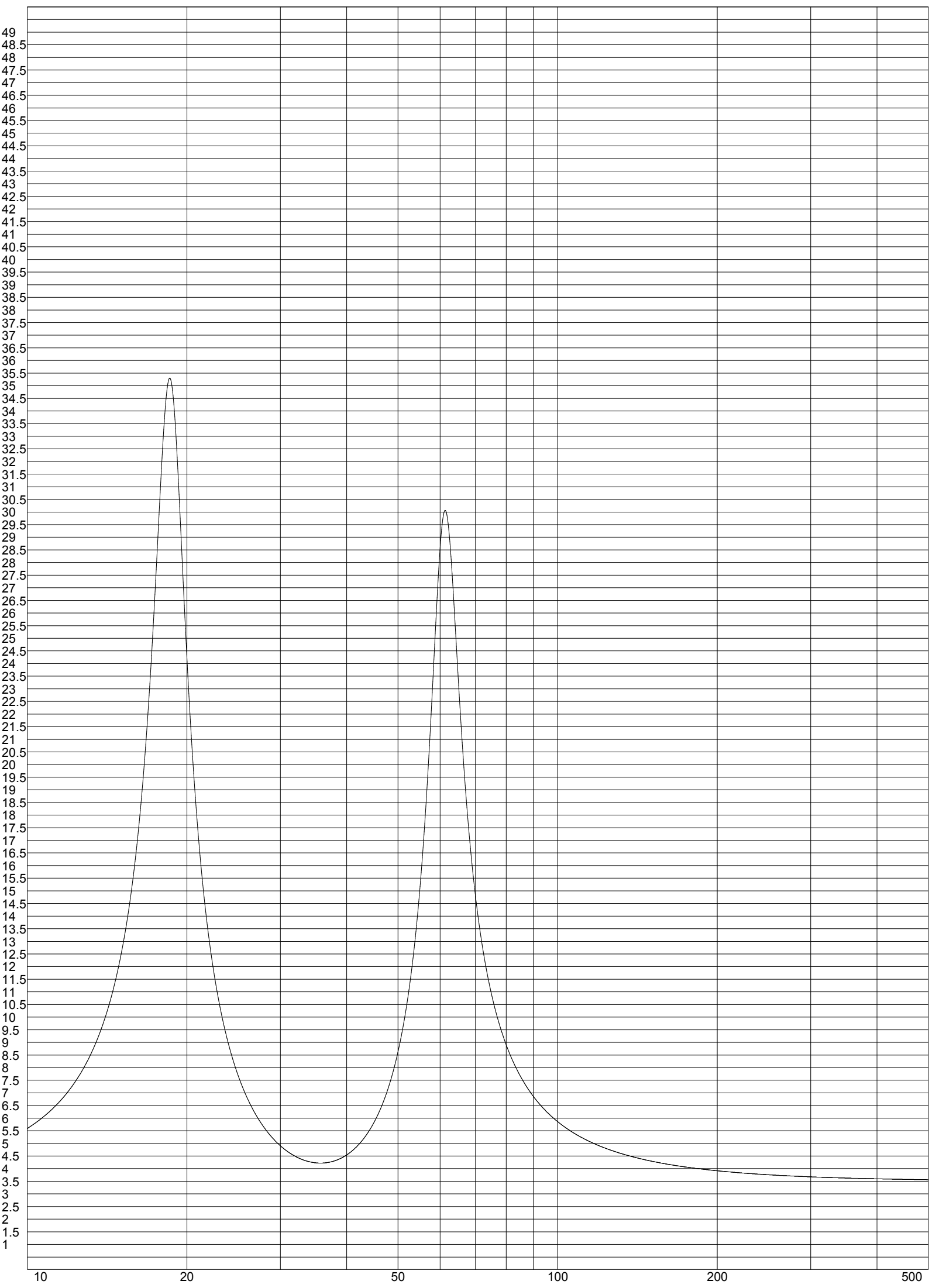
Impedance [ohm] - [1]Vented : Iwai 125 Watts
