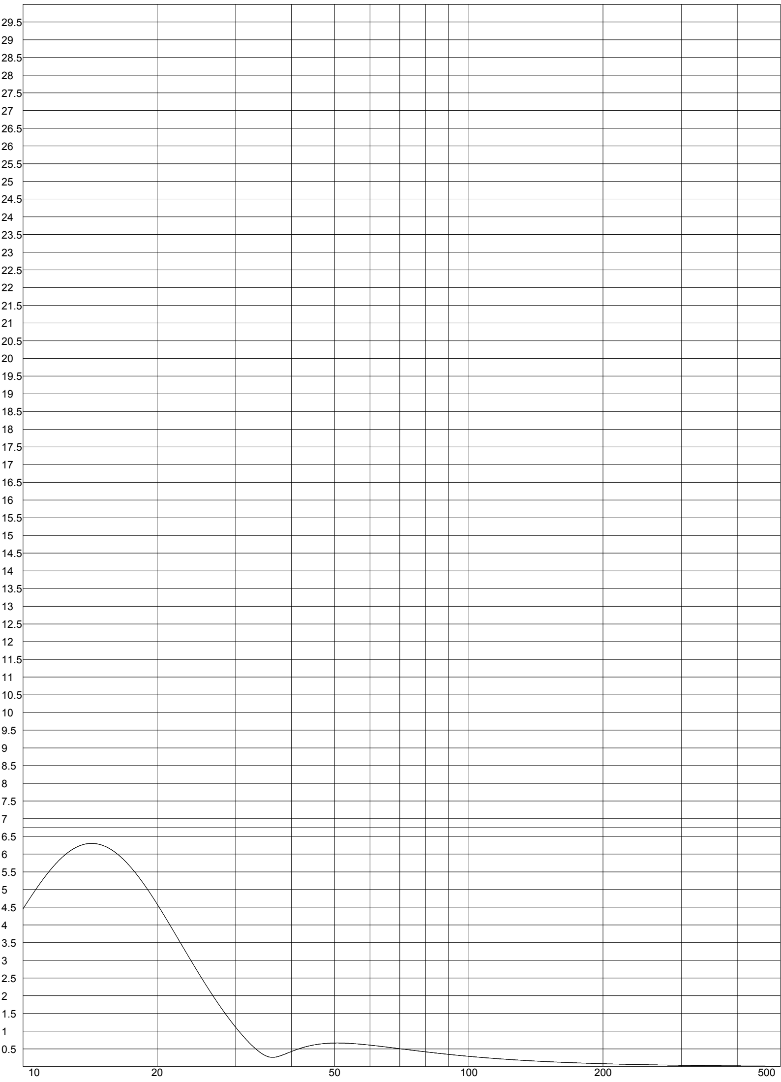
Cone excursion [mm peak] - [1]vented : Iwai 125 Watts
