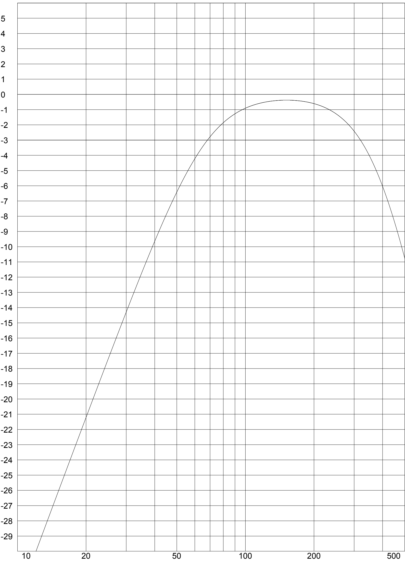
Transfer function magnitude [dB] - [1]Closed : Iwai 125 Watts
