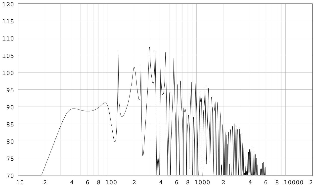
----- SPL RESPONSE [DB] - CONSTANT DIRECTIVITY -----
