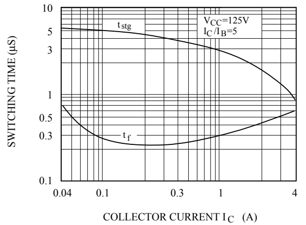
SWITCHING CHARACTERISTIC
