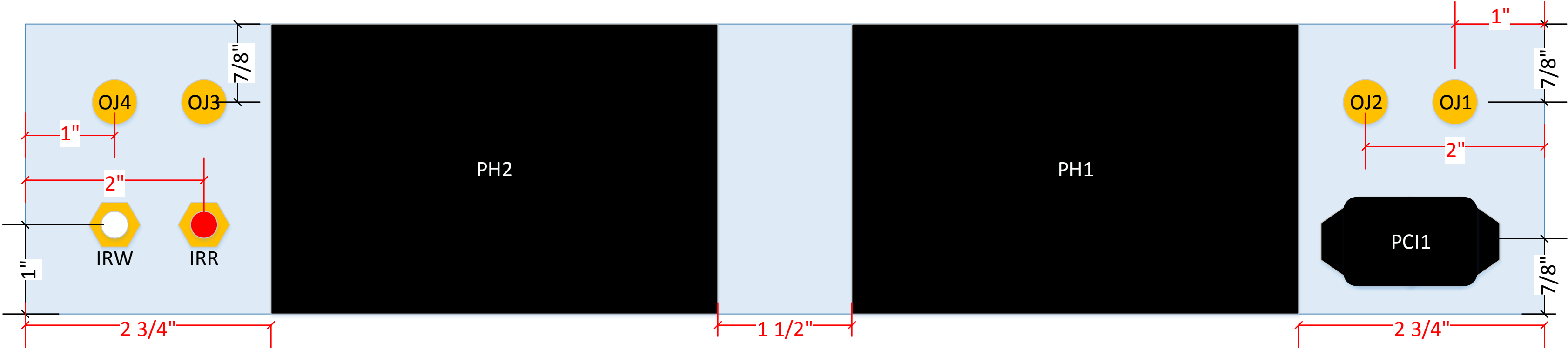
View from outside, rear of amplifier
