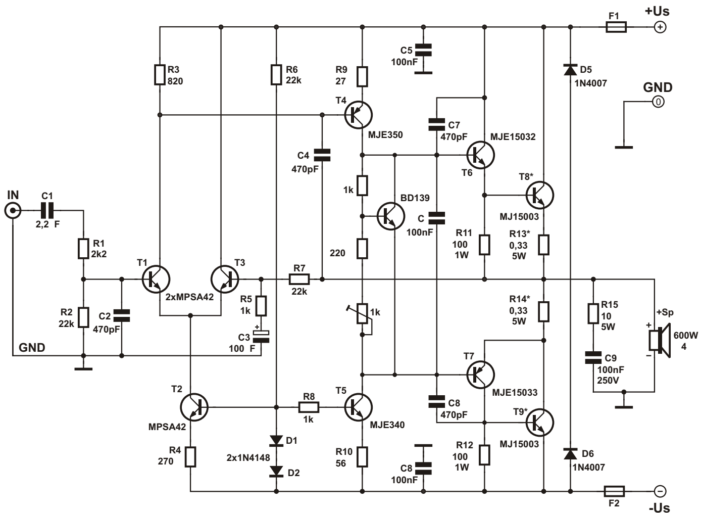
Figure 1. (class-AB 500W Amplifier)
