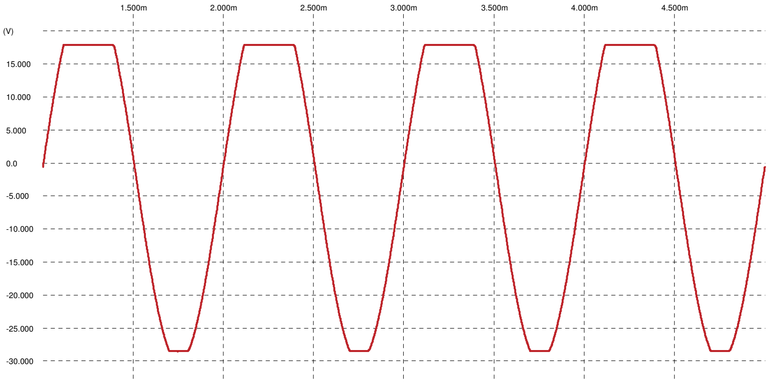
memdist power-Transient-8-Graph
