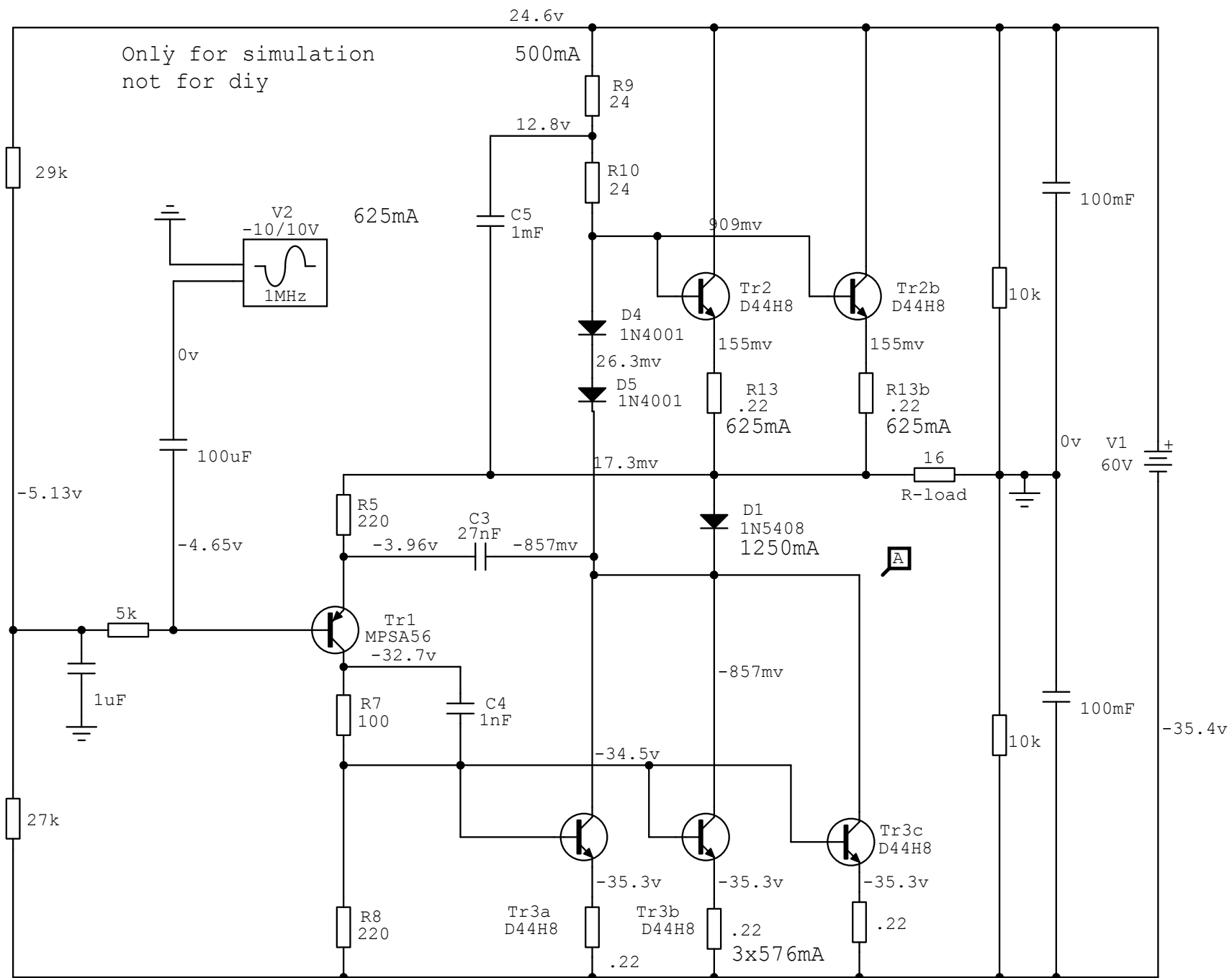
composite collector... (single ended buffer stage) based on Ollson III and http://www.diyaudio.com/forums/showthread.php?s=&threadid=72149
