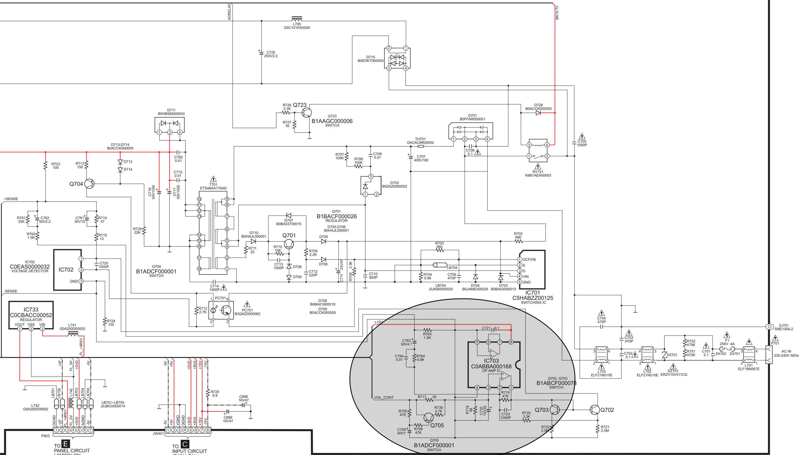
SA-XR57E/EB/EG POWER CIRCUIT
