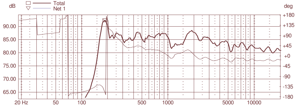
Summed frequency response
