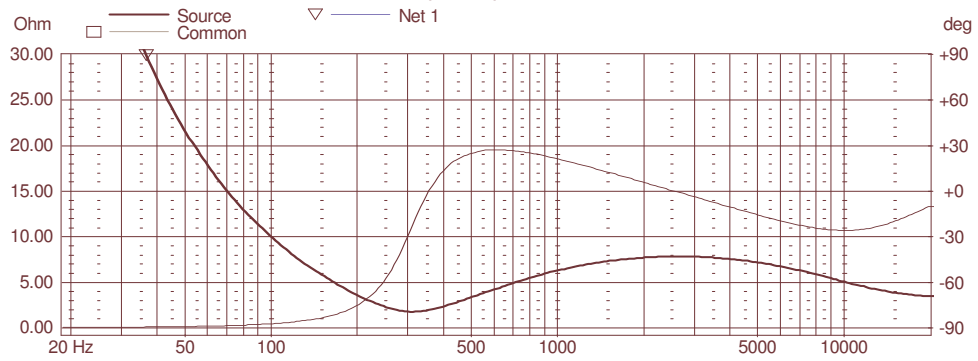
Input impedance
