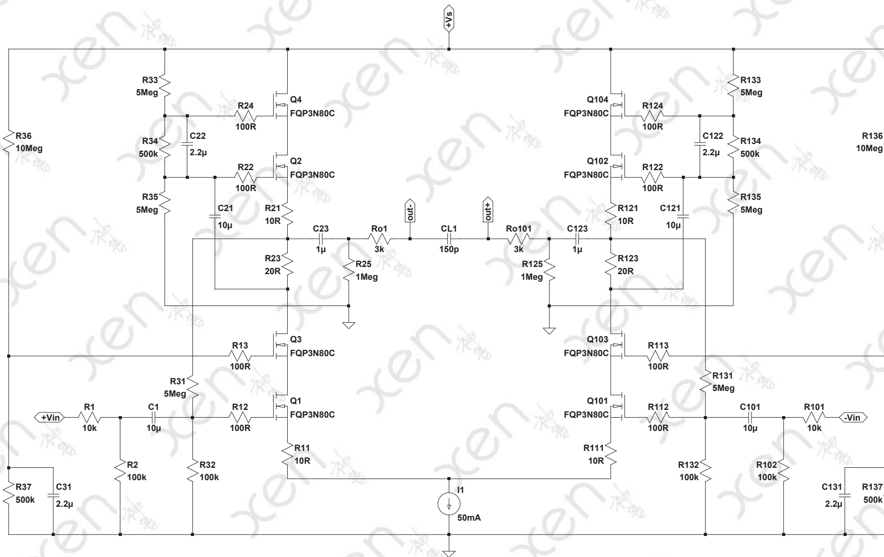
Pass STAT Headamp Concept w. Cascoded MOSFET Version 1.0 Dec 2013
