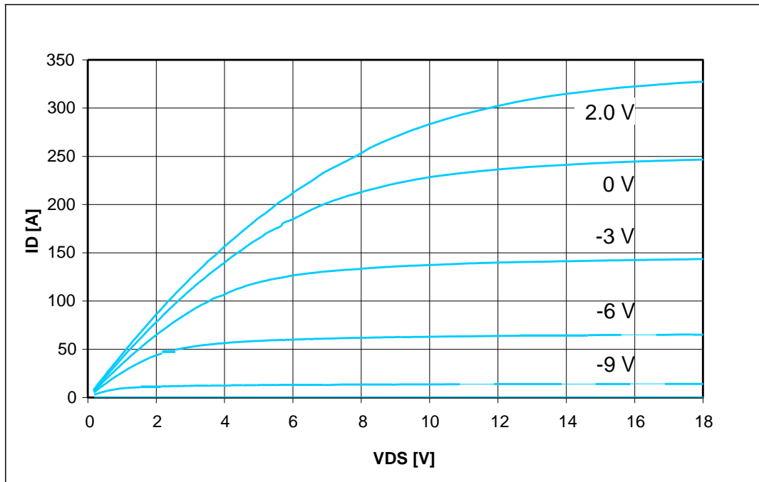
Fig. 3: Typical output characteristics of a 35mOhm rated 1200V JFET at 25°C, parametrized by the gate-source voltage.
