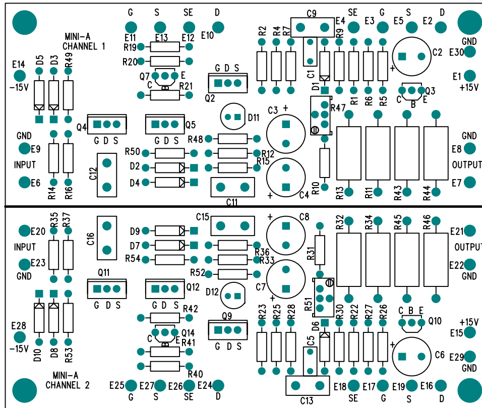
PRIMARY SILK SCREEN
