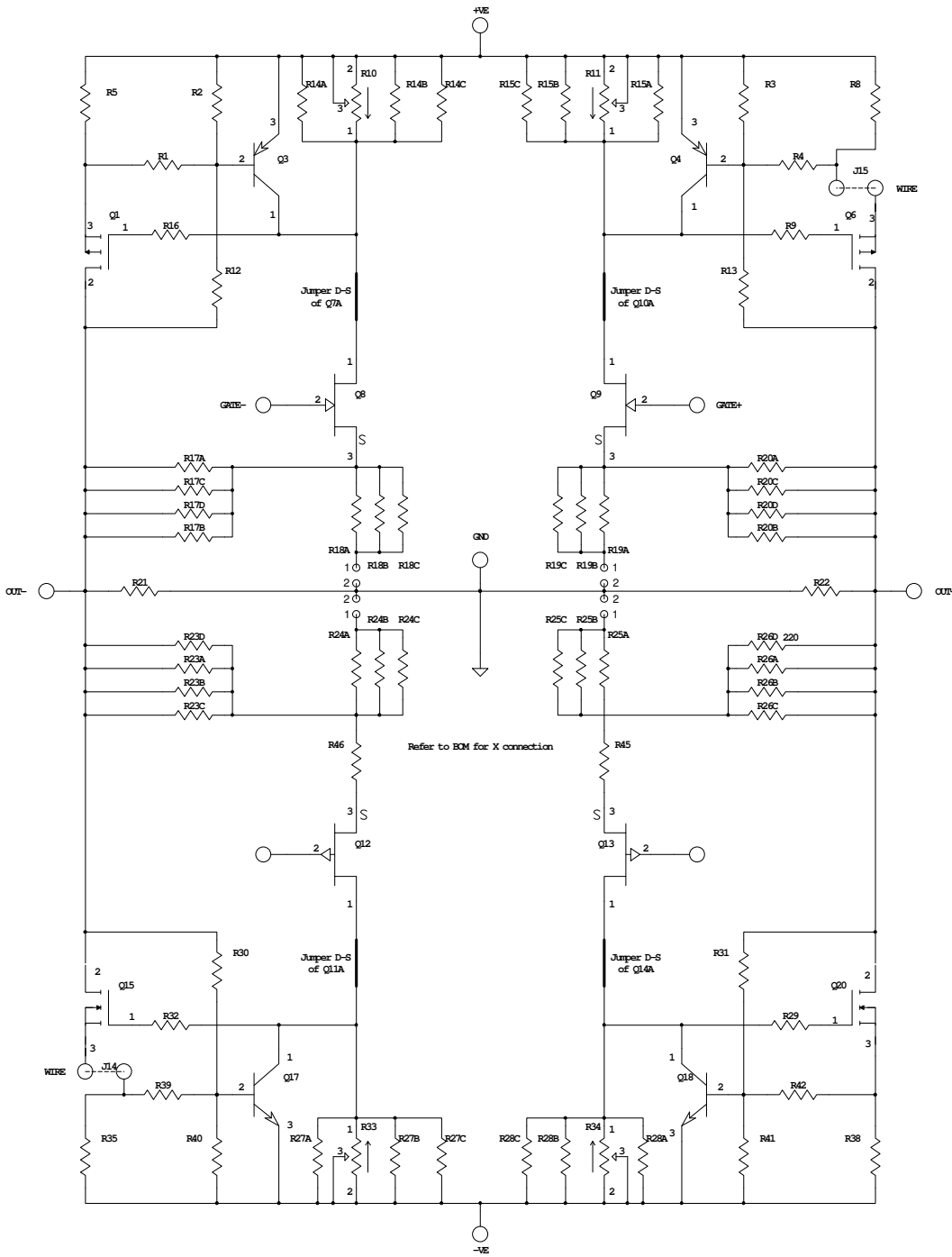
F5X Balanced Power Amplifier Standard Configuration Version 1.0 XEN Audio 2011
