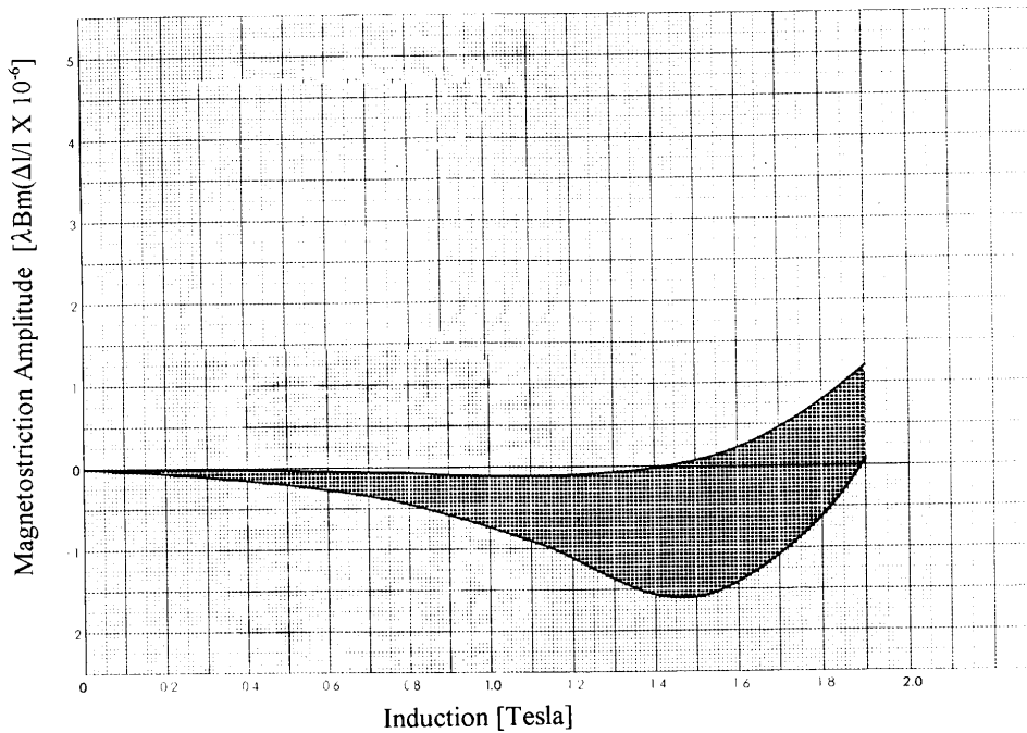
Figure 5: AC magnetostriction: the Magnetostriction Amplitude is shown versus the AC induction in Tesla. (reference [9])
