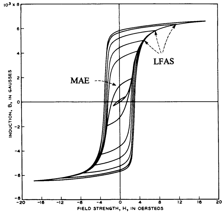
Figure 4: MAE occurs in the steep section of the hysteresis loop. Rotation and LFAS are dominant near saturation in the hysteresis loop.
