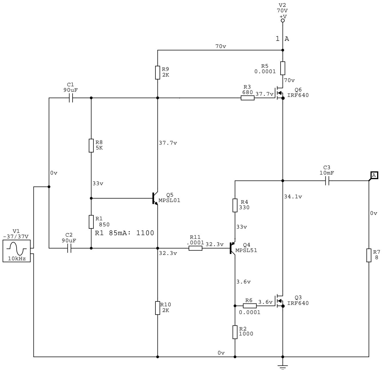
Output power buffer of MOSFET 12 (page 65/66 Fig. 6/8) the quasi complementary version from the book "Power Amp Projects" (collection of released amp projects in Audio Amateur 1970 - 1989)
