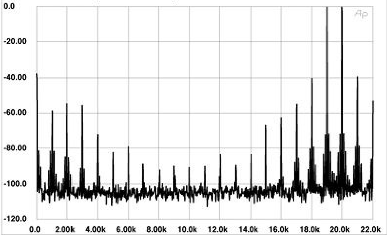
STEREOPHILE Pass Aleph 3 HF intermod spectrum at 26.7W into 4 ohms dBr vs Hz
