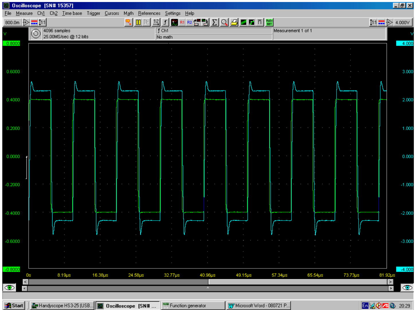
100kHz Square Wave (RHS) Input Green, Output Cyan
