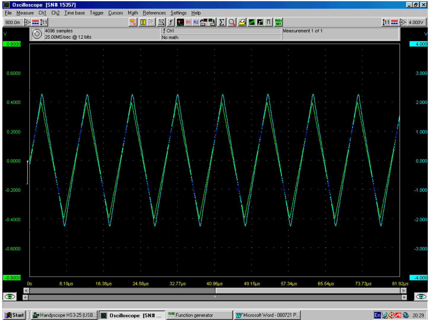
100kHz Triangular Wave (RHS) Input Green, Output Cyan
