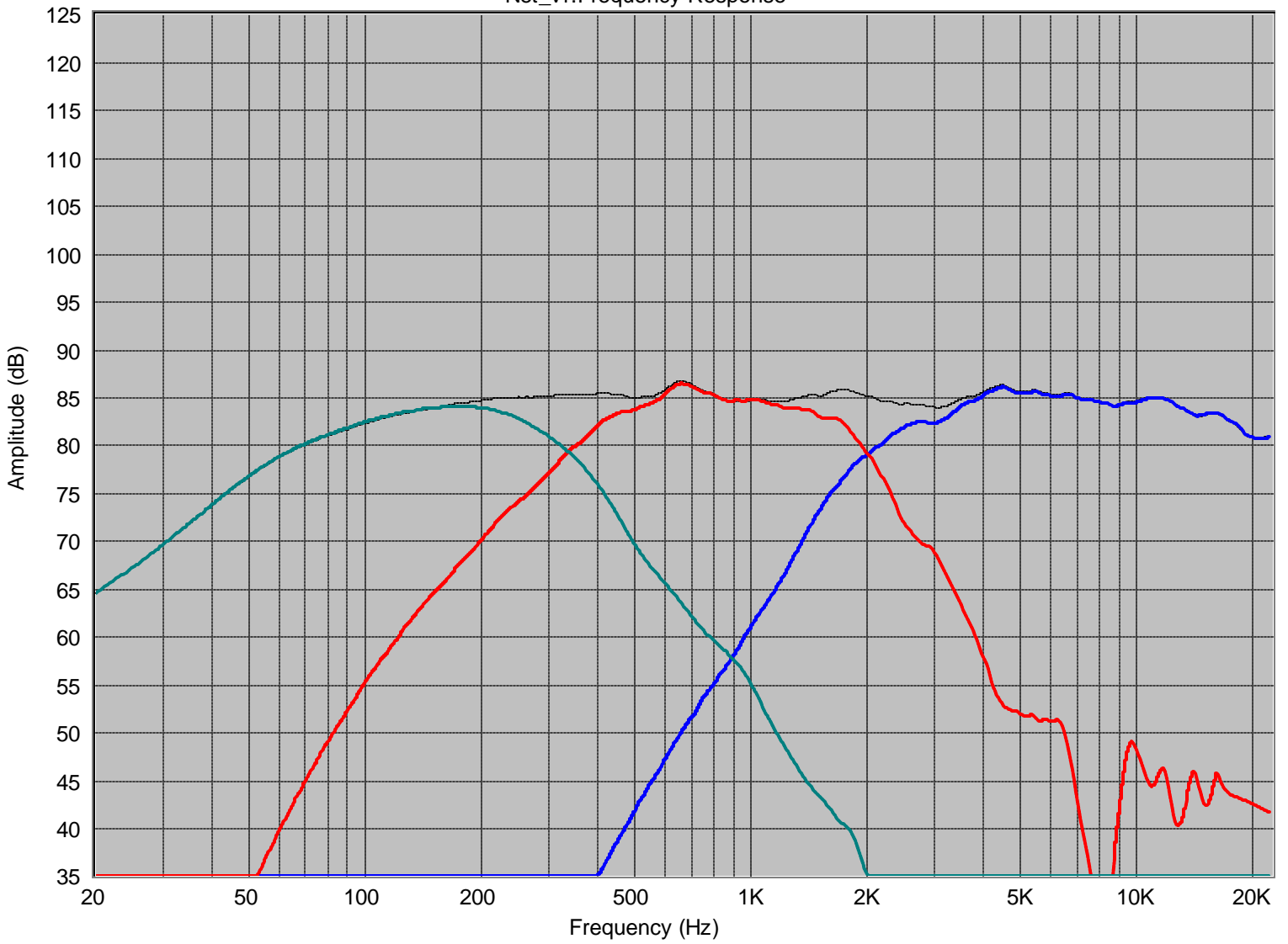
Net_v1.Frequency Response
