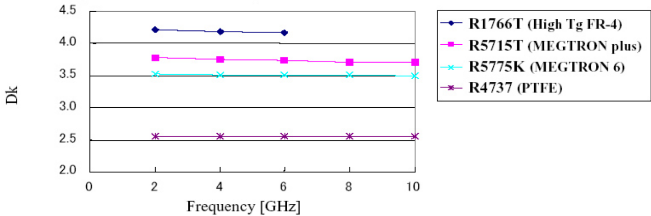
Dk/Df (IPC TM-650 2.5.5.5)
