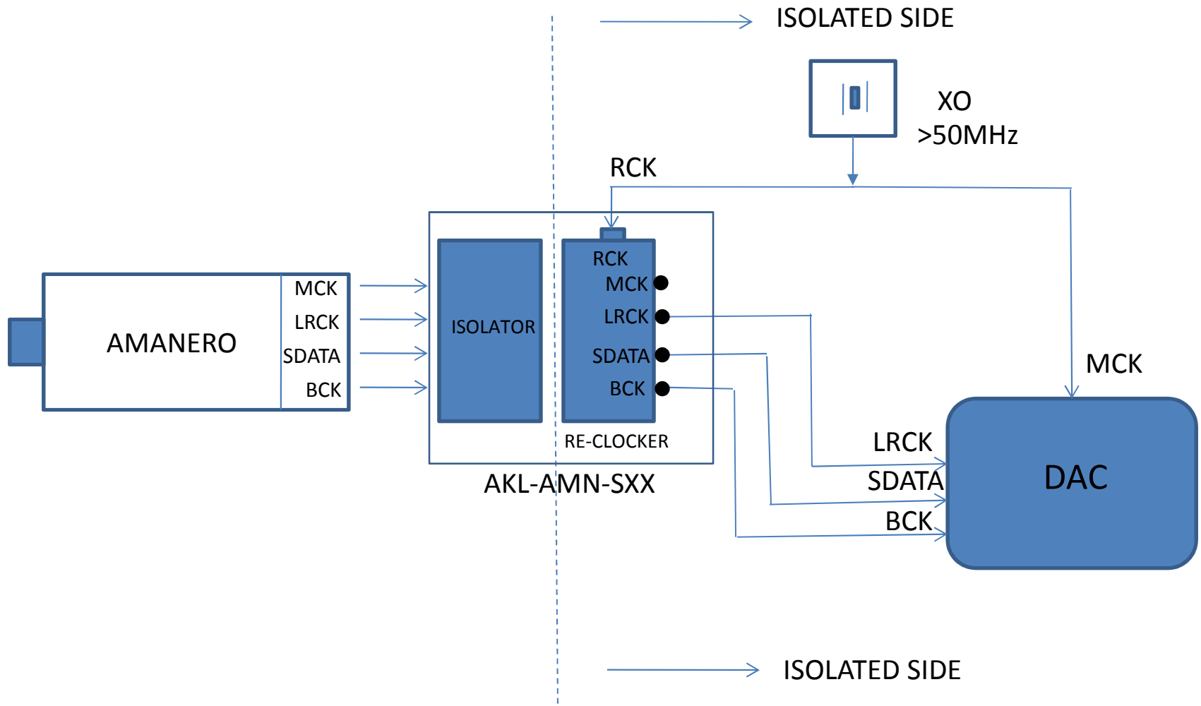
Isolated Connection with Re-Clocking – Pseudo Sync Mode (Common Clock)
