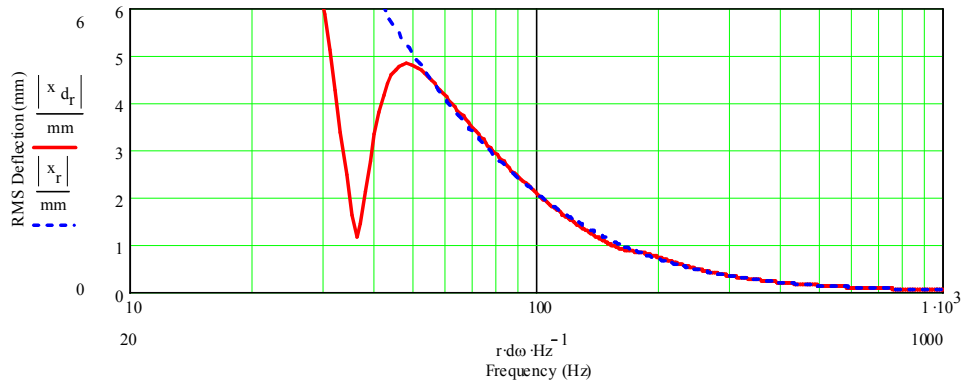
Woofer RMS Displacement (15 Watts Input)
