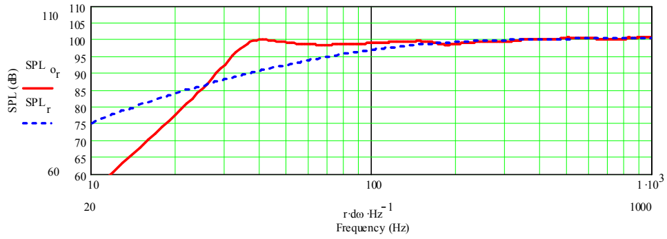
System Far Field and Infinite Baffle SPL Responses (15 Watts Input)
