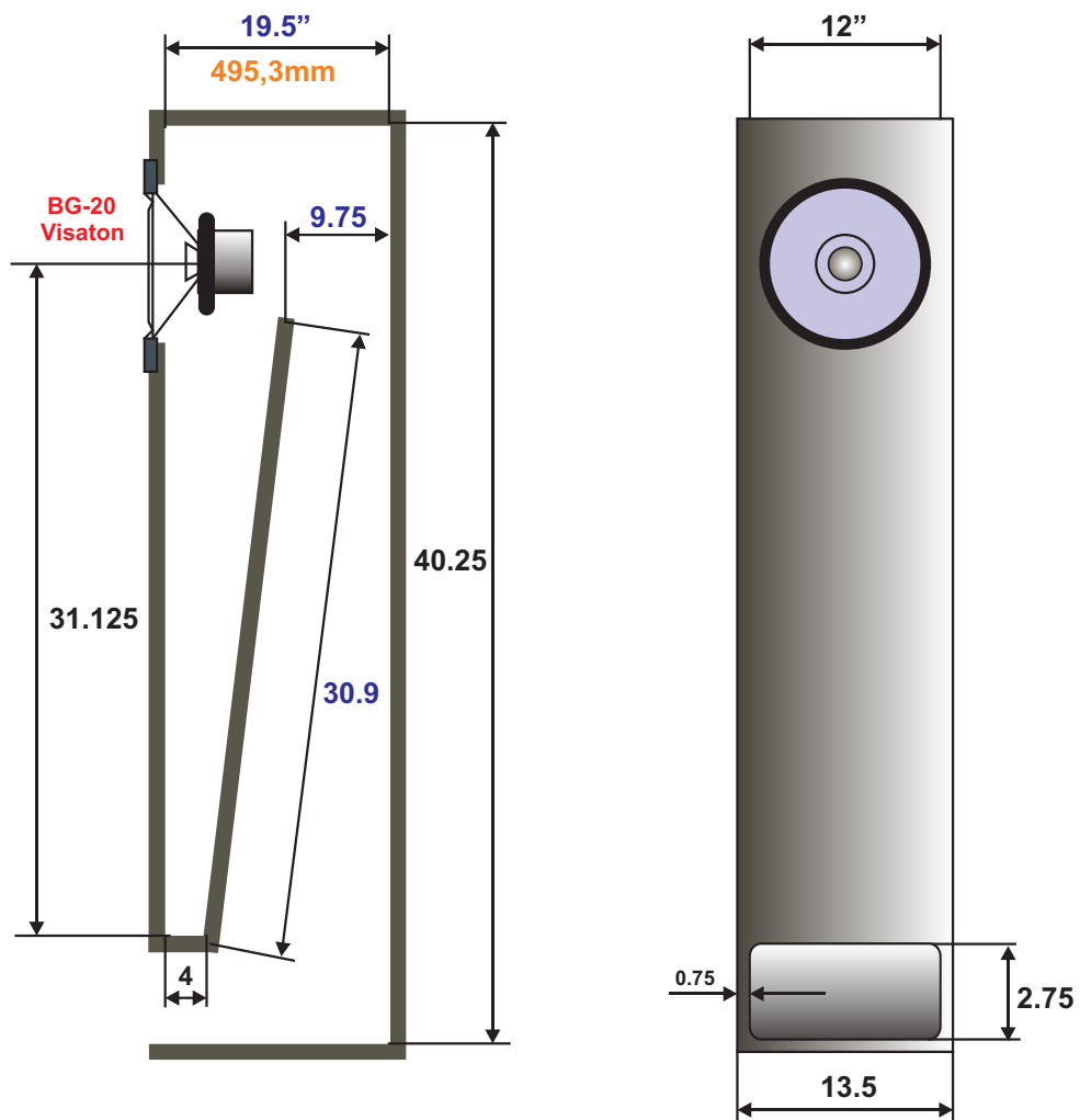
Cabinet for speaker BG-20 Visaton (1"=25,4mm)
