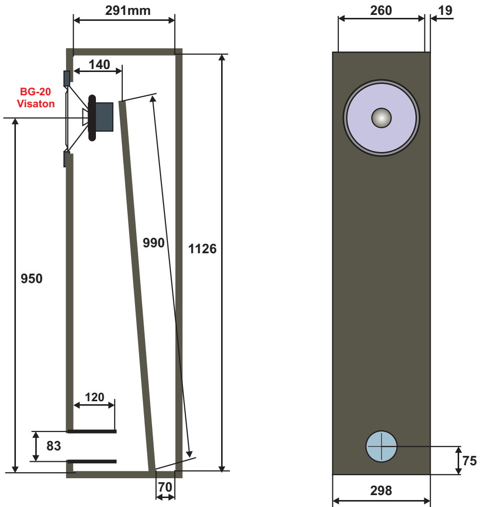
TQWT-cabinet for speaker BG-20 Visaton
