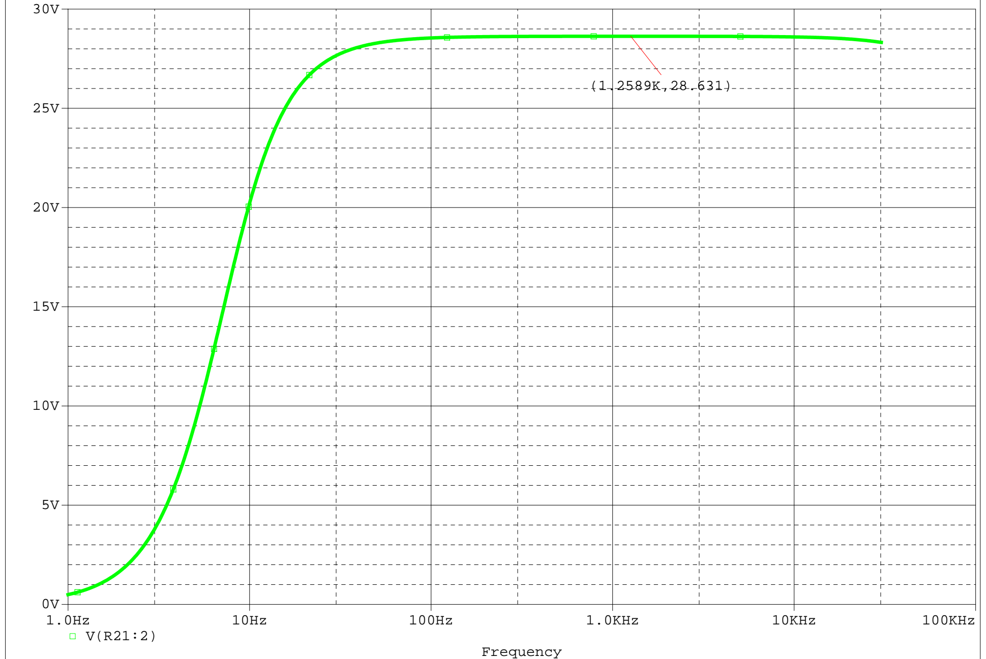
(A) Bode.dat (active)
