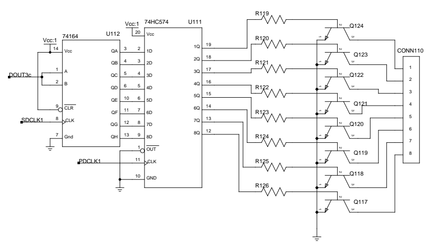
Relay board drivers
