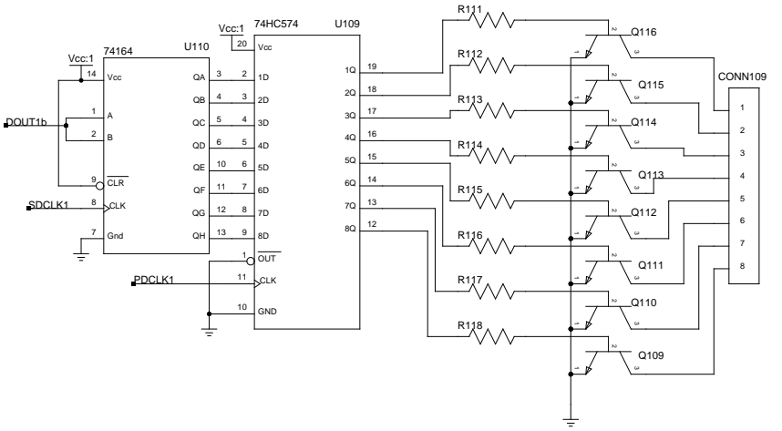
Relay board drivers
