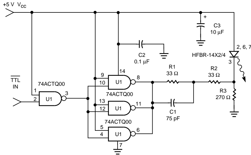
Figure 18b. 155 Mbd Fiber-Optic Transmitter for TTL Interface.
