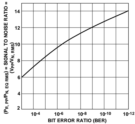
Figure 13. Signal-to-Noise Ratio vs. Probability of Error.
