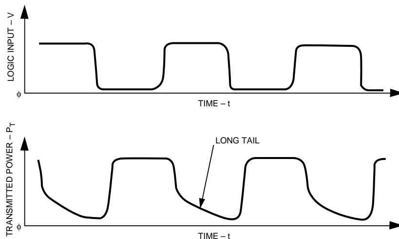
Figure 4. Example of Long-Tailed Response.
