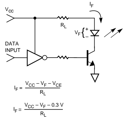
Figure 5. Series Switch LED Driver.
