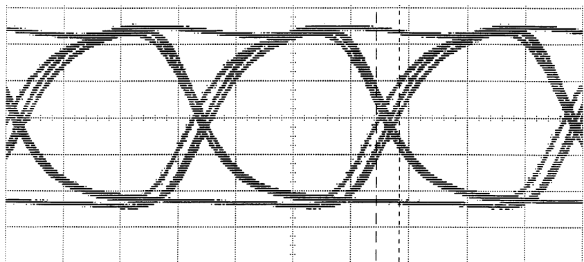
Figure 9. Optical Output of the TTL Transmitter.
