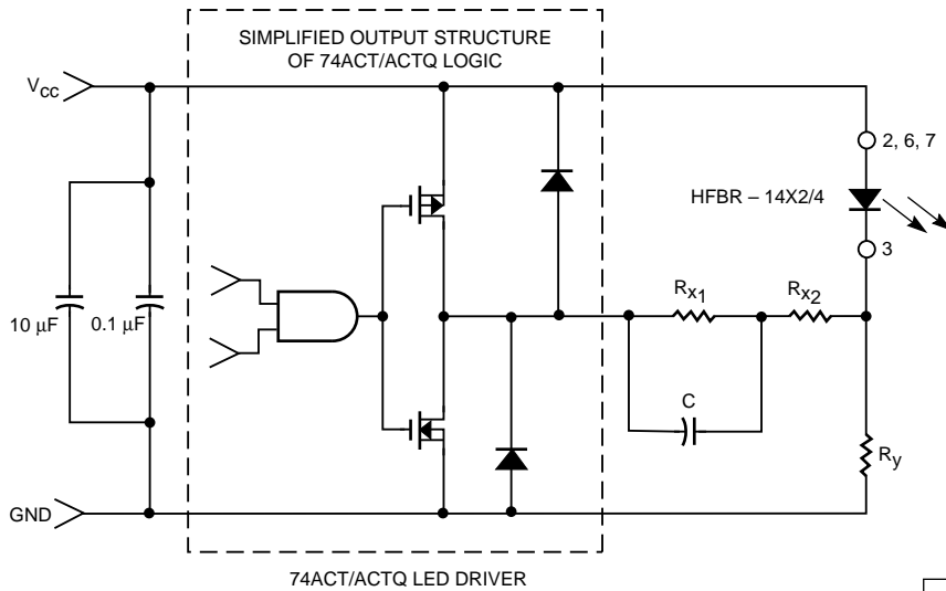
Figure 6. Simple High-Speed Transmitter Circuit.
