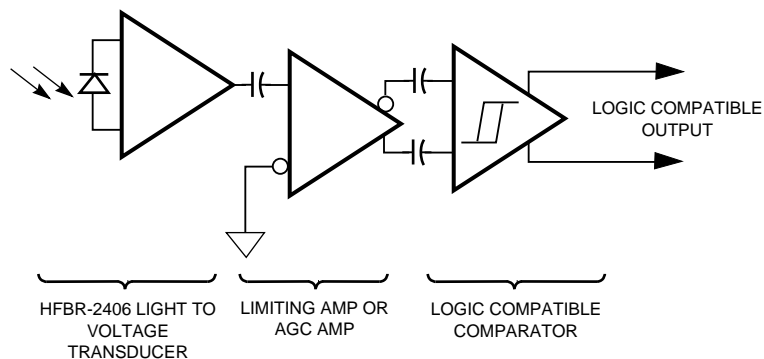
Figure 12. Fiber-Optic Receiver Block Diagram.
