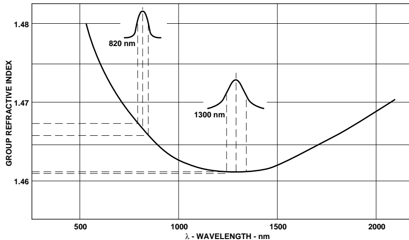
Figure 1. Group Delay vs. Wavelength.
