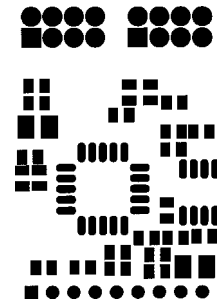
Figure 23c. Top Side Solder Mask
