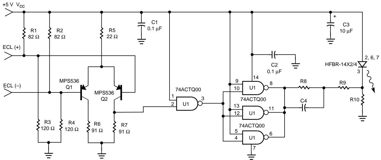
Figure 10. Transmitter with +5 V ECL Interface.
