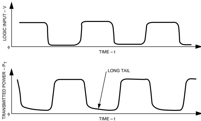
Figure 7. Improved Optical Output Waveform.
