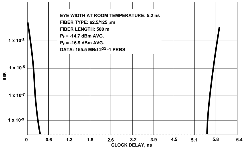
Figure 20. Typical BER vs. Clock Delay at 155.5 MBd.
