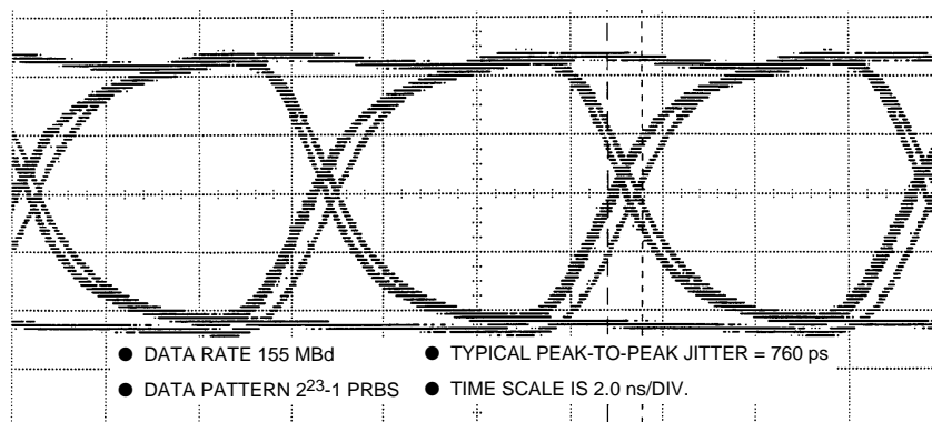
Figure 11. Optical Output of the +5 V ECL Transmitter.
