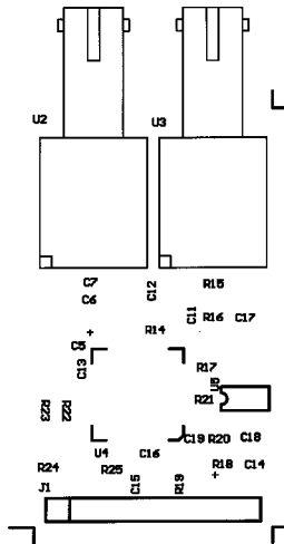
Figure 23b. Top Silkscreen
