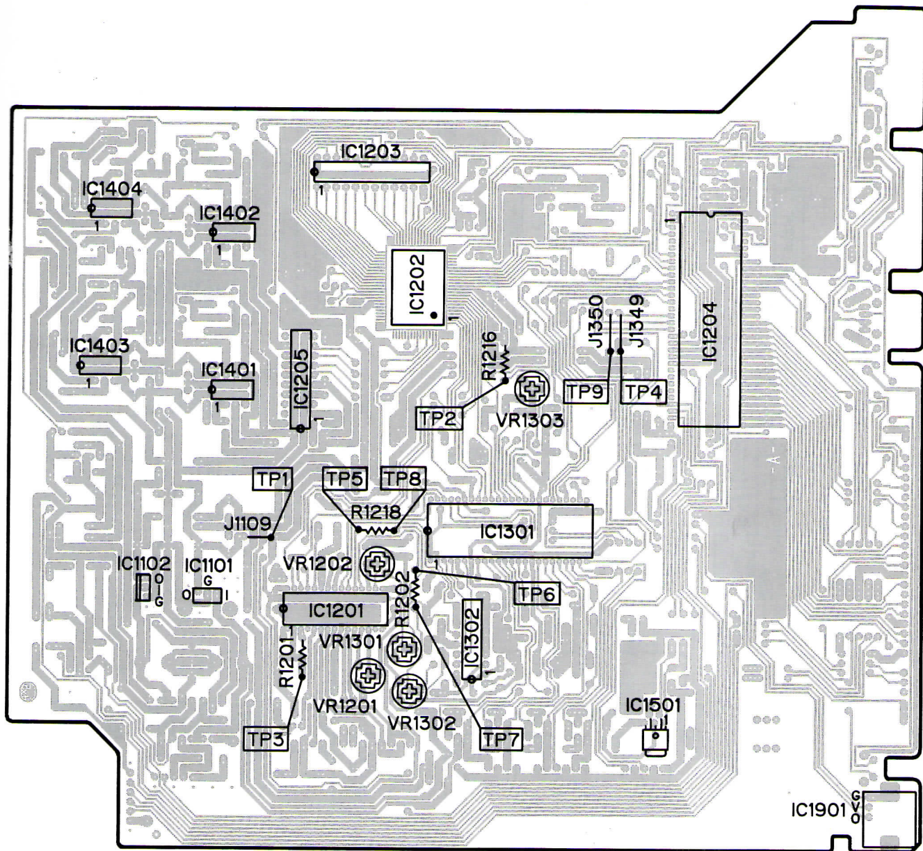
Figure 21. Main P.C. Board (Component Side)
