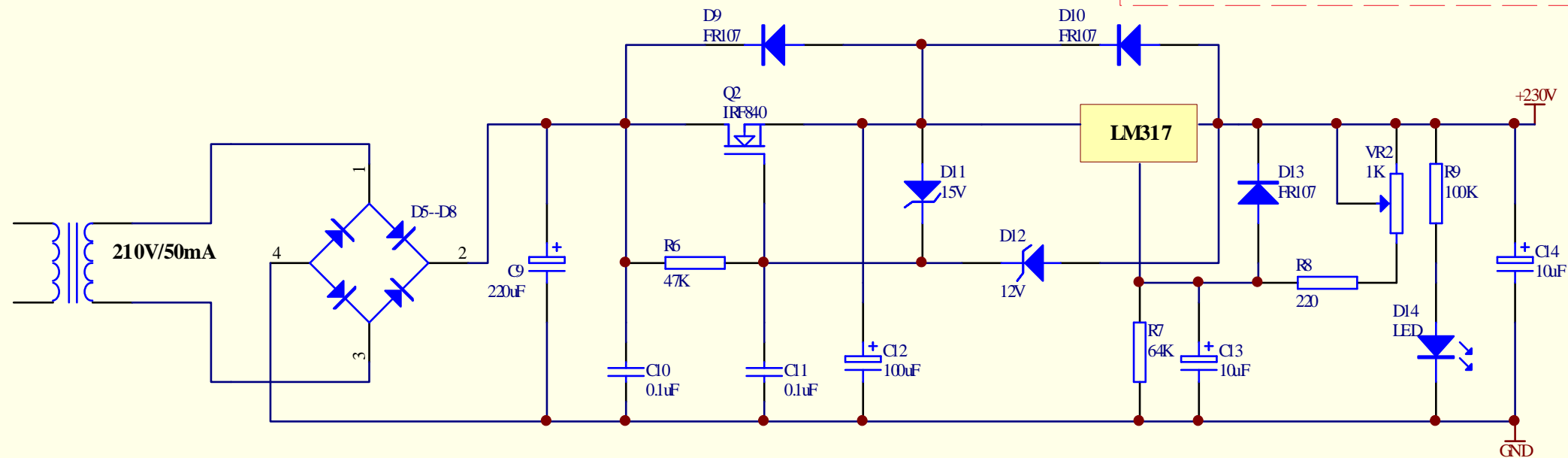
DC2-SCH
