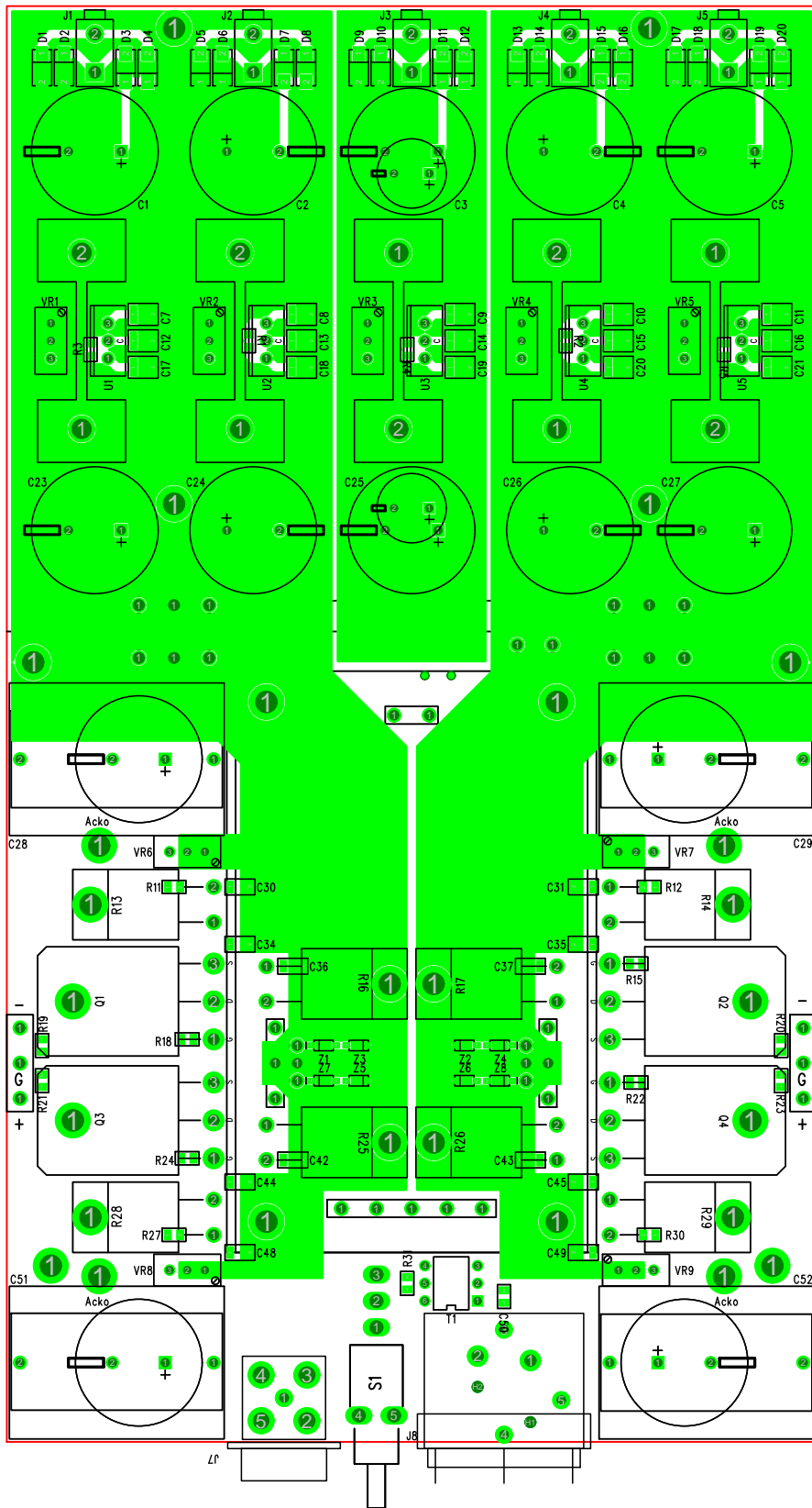
D1B1 - IV STAGE - 02/2010 SILKSCREEN (TOP SIDE)
