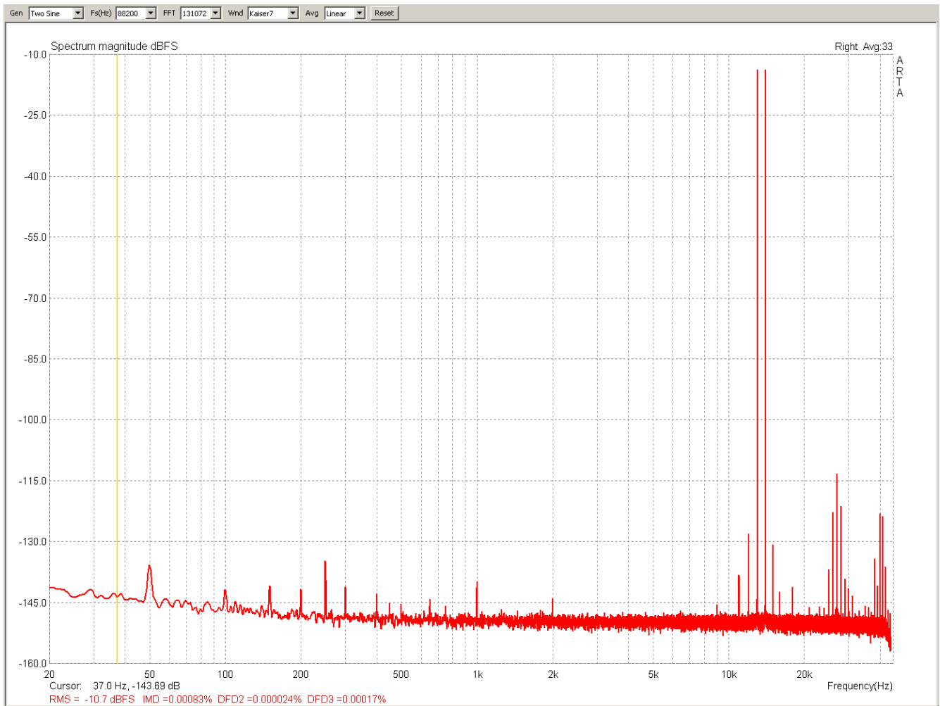
FE – V7 – 5W – IMD test: 13-14kHz
