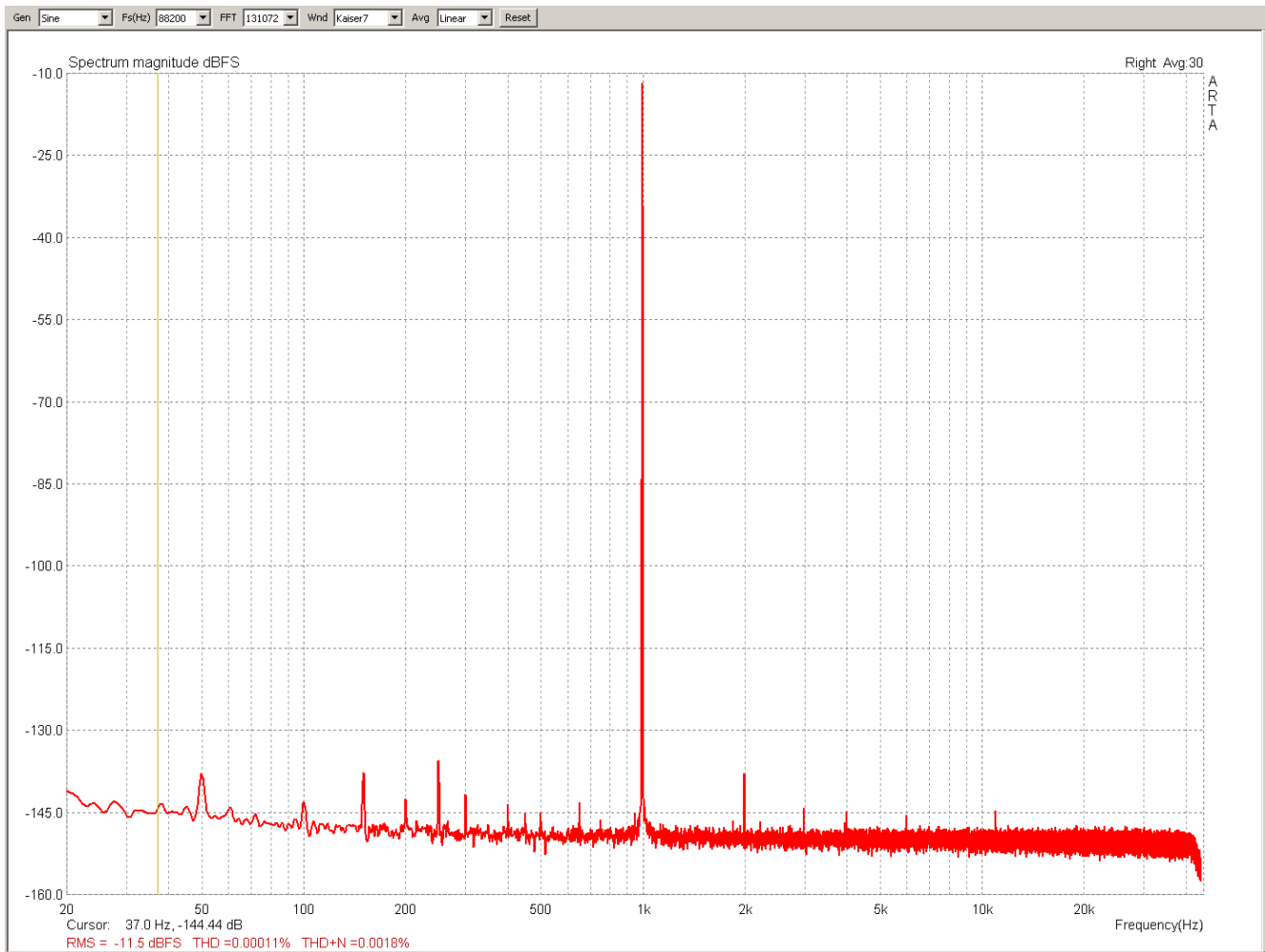
FE -V7 – 5W ( 6.2VRms – 6.8ohmload) 1KHz THD
