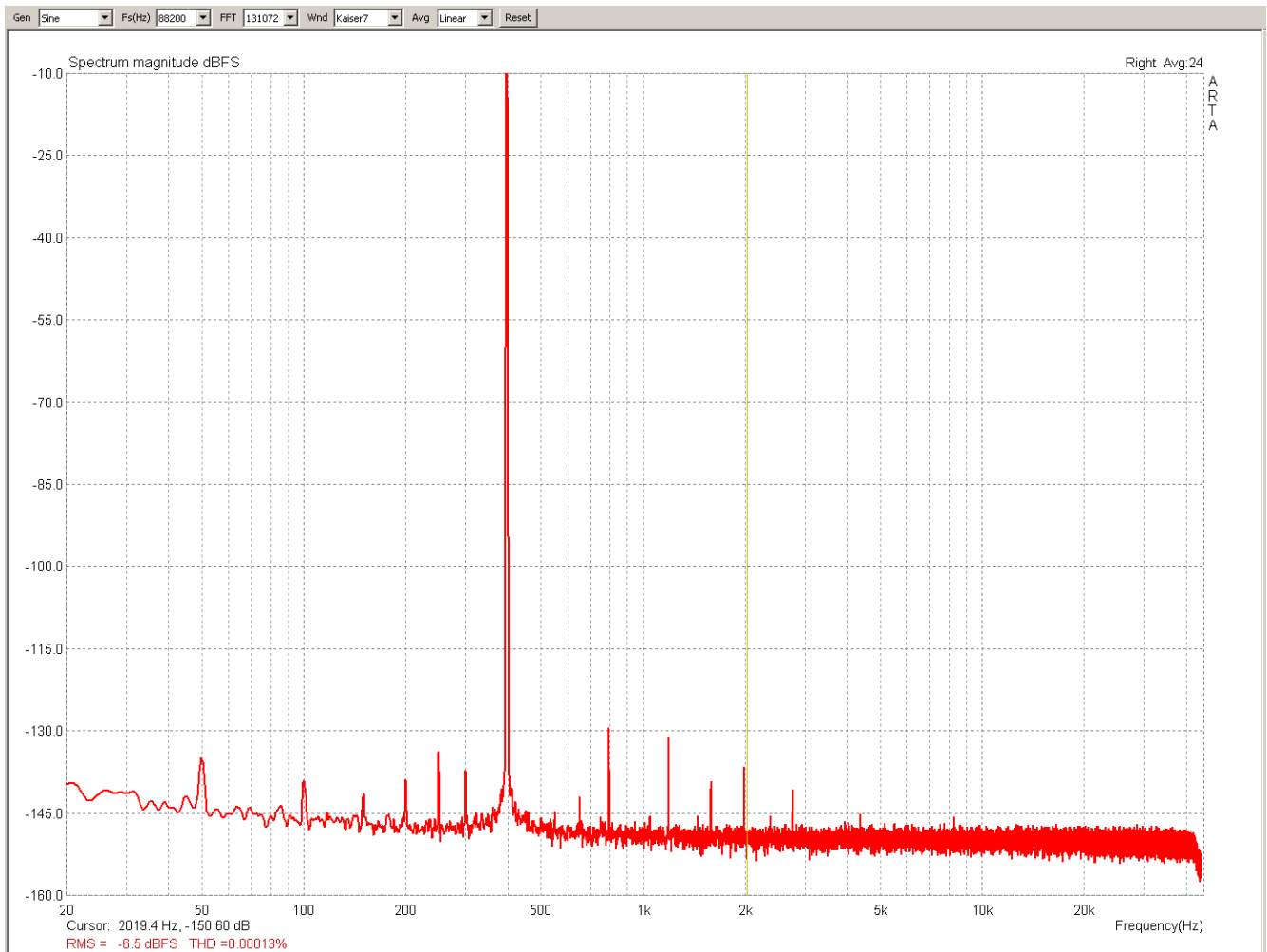
FE - V7 -18W (11.8VRms -6.8ohm) – 400Hz THD
