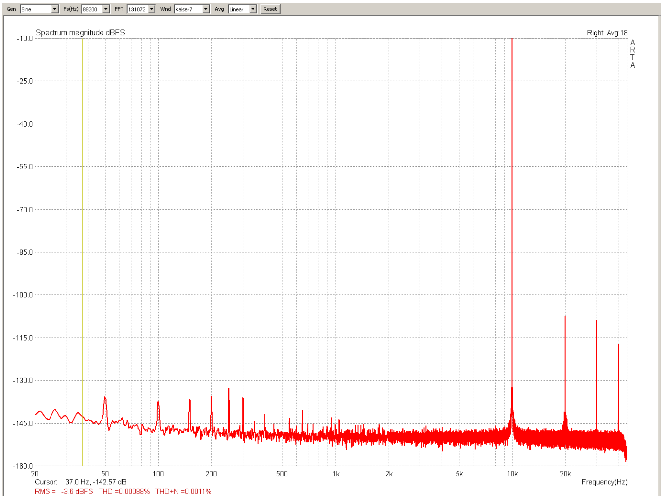
FE - V7 - 40W (16.5VRms -6.8Ohm Load ) – 10kHz THD
