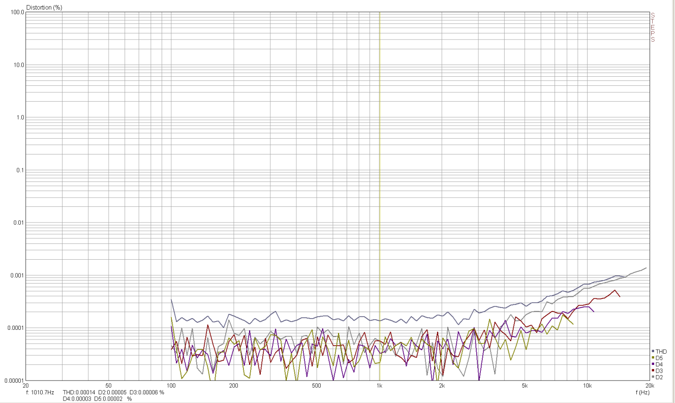
FE -V7 - 5W - distortion versus frequency sweep
