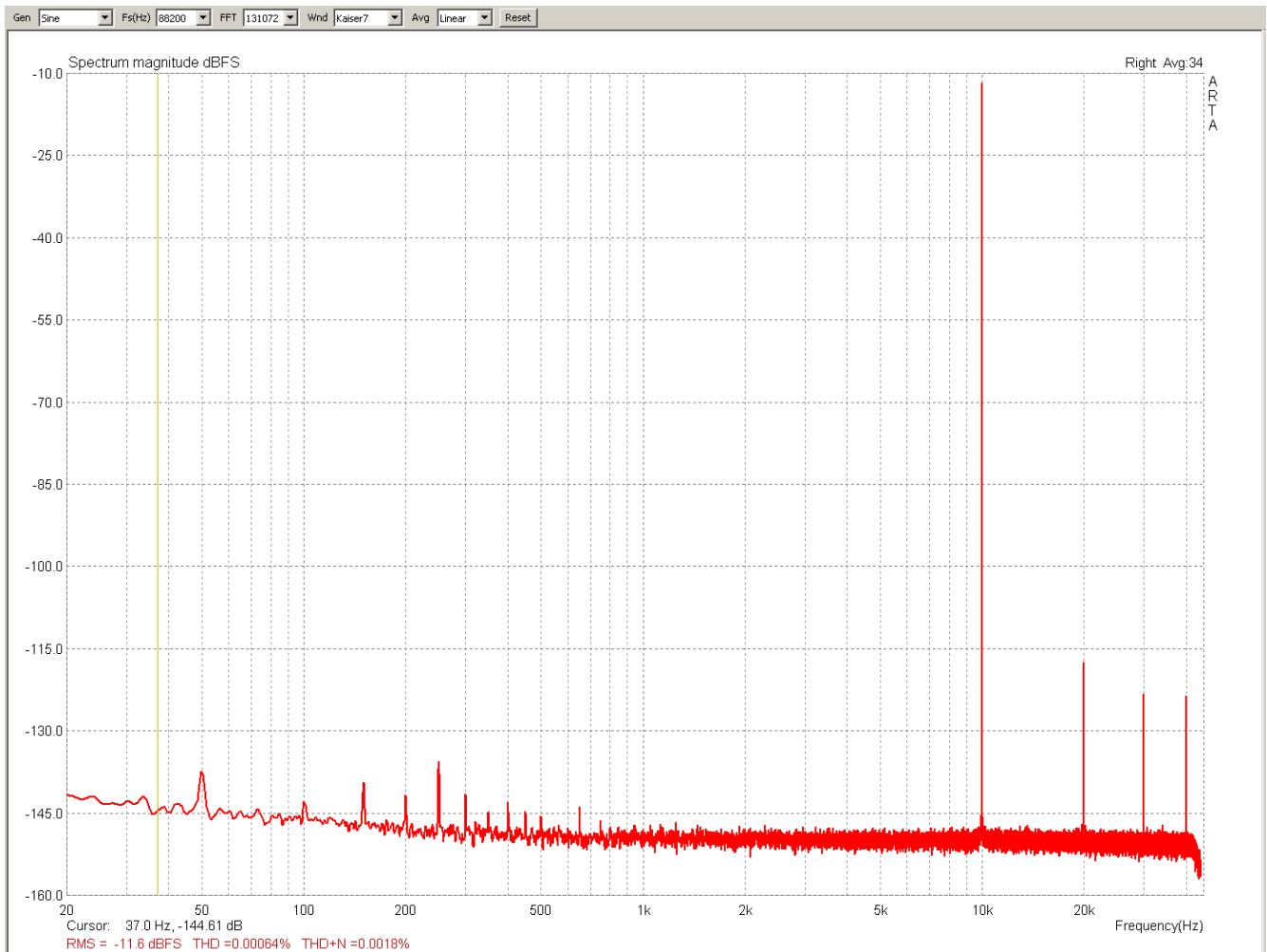
FE-V7 - 5W - 10kHz THD
