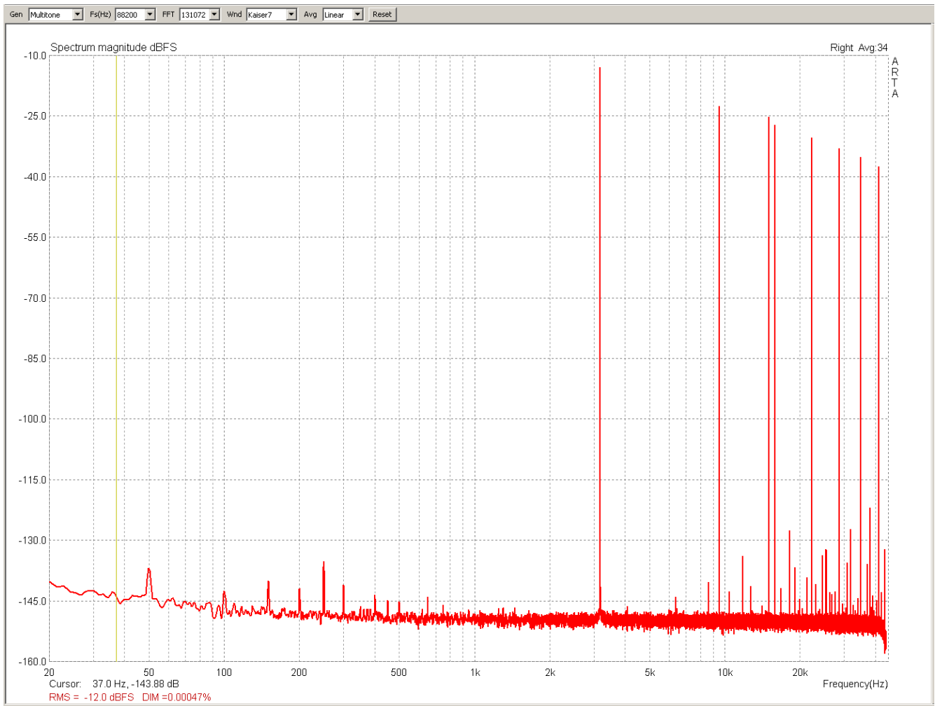
FE -V7- 5W – Dynamic InterModulation test
