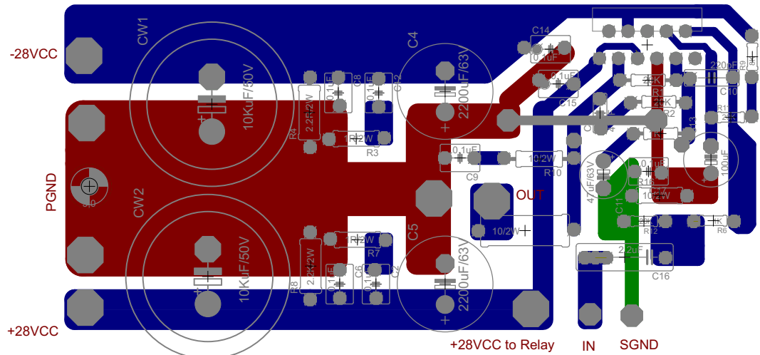
Power Amp
