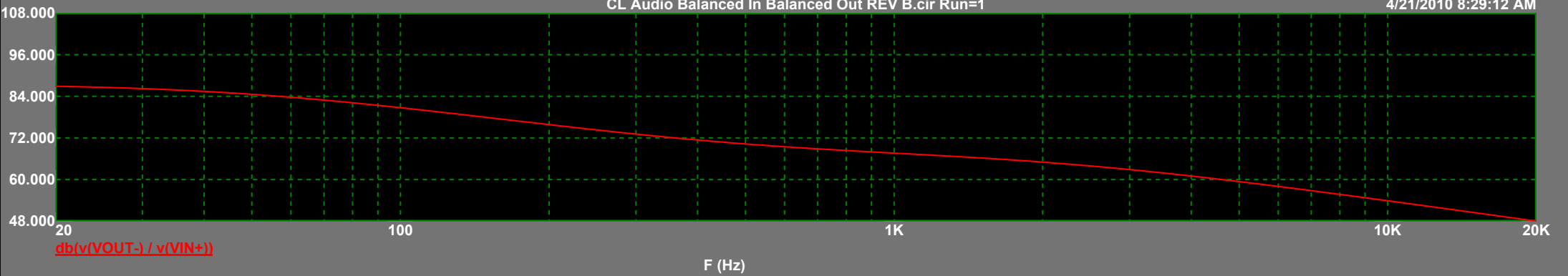
CL Audio Balanced In Balanced Out REV B.cir Run=1
