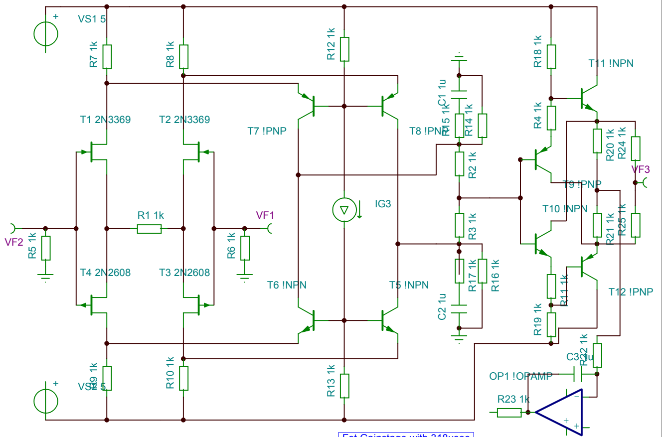
Fet Gainstage with 318usec and 3180usec Riaa and open loop Diamond buffer and servo
