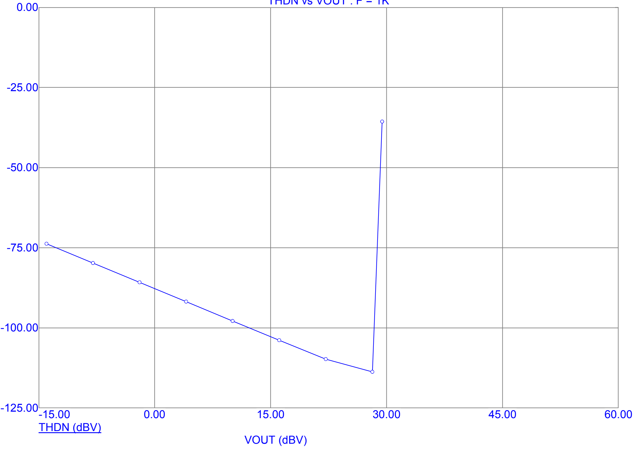
THDN vs VOUT : F = 1K
