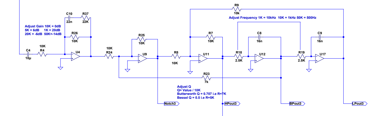
2nd Order State variable filter independent gain and Q with notch output.
