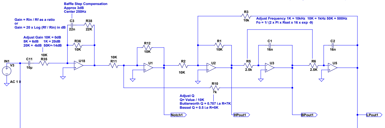
2nd Order State variable filter independent gain and Q with notch output.
