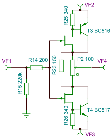
High Speed Low Distortion Buffer Fets : 2SK170, 2SJ74 BC516, BC517 are Darlington
